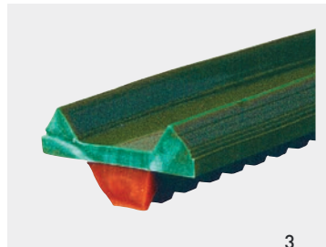
Flat belt with a trapezoidal profile below and SF7 walls above.
